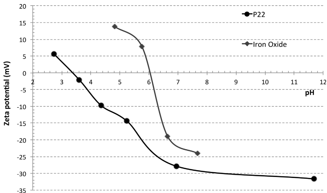
Fig. 2. Zeta potential as a function of pH for: P22 bacteriophage, ionic strength 15 mM of NaCl, T = 20 \text{ }^\circ\text{C} ; and nanostructured iron oxide, ionic strength 15 mM of NaCl, T = 20 \text{ }^\circ\text{C} .
