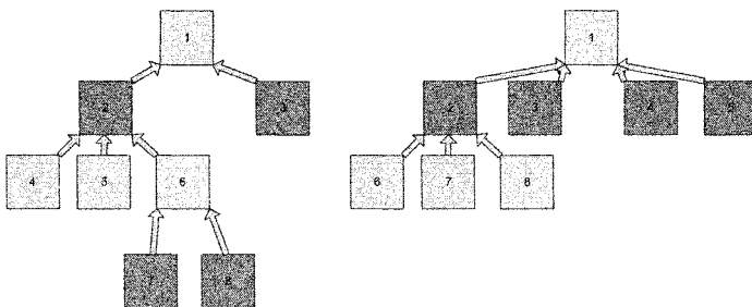
Fig. 1. Decision trees
