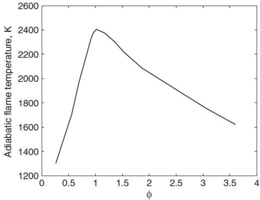
Figure 2.2.3: Adiabatic flame temperature for hydrogen-air-mixtures [54]
