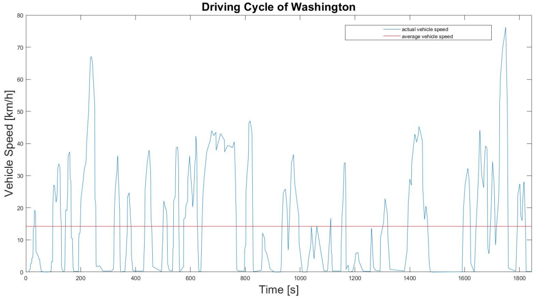
Figure 3.2.3: WMATA-Cycle
