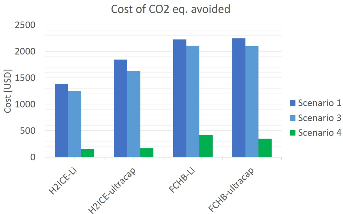
Figure 5.5.1: Costs in US$ per saved ton of global greenhouse gases
