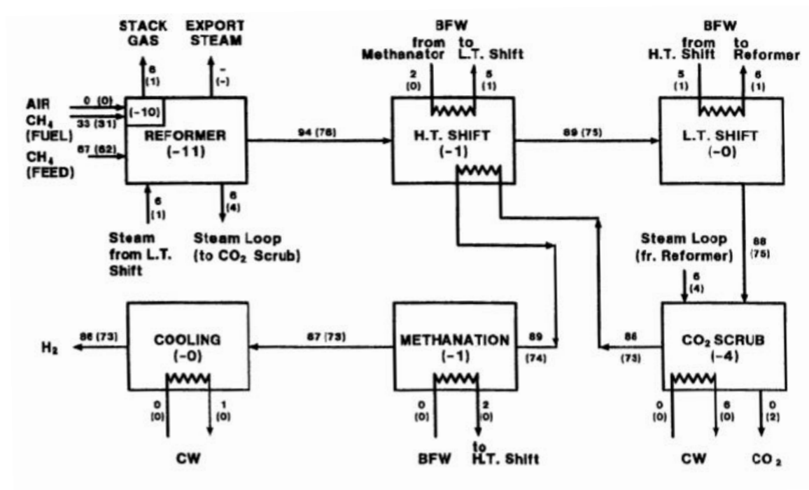
Figure 2.1.2: SMR [49]
