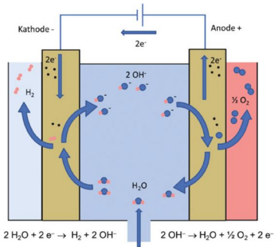
Figure 2.1.3: Electrolysis [32]
