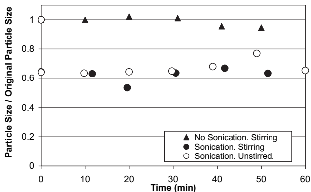
Fig. 3 – Influence of stirring and sonication in particle size over time.
