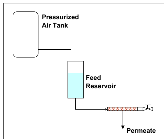
Fig. 1 – Operational setup.
