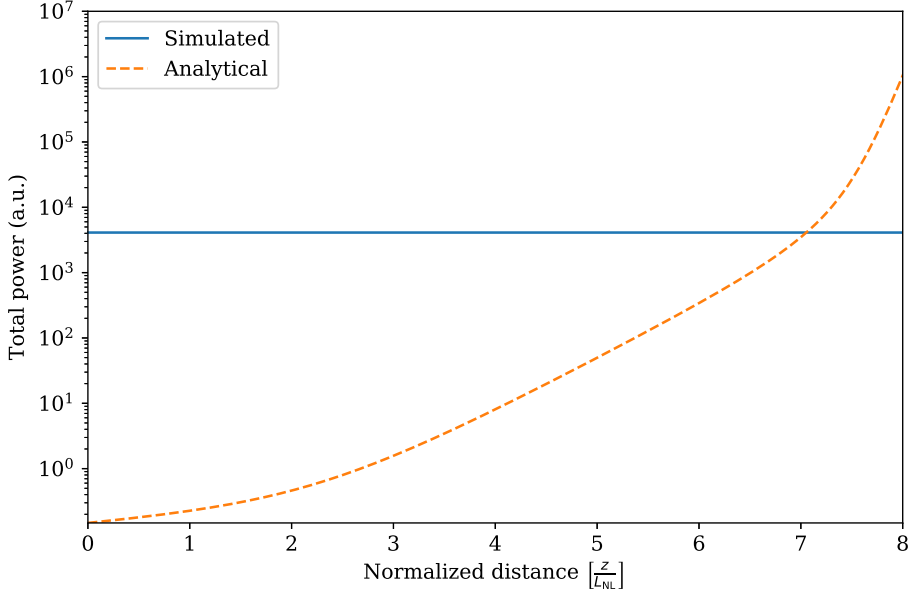
Fig. 4. Total signal power for the analytical approximation (dashed line) vs. simulation (solid line). The crossing at nearly 7 L_{NL} (cf. Fig. 3) marks the maximum propagated distance at which the analytical approximation remains valid.
