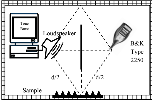
Fig. 6. The geometry environment with angles
