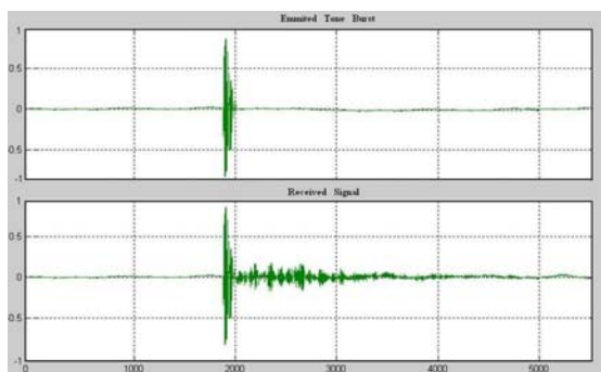
Figure 4. Emitted Tone Burst and Received Signal
