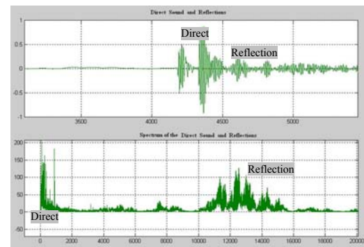
Fig. 5. The Direct and Reflect Sound
