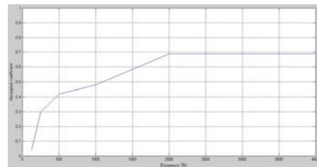
Fig. 7. Absorption Coefficients in octave bands
