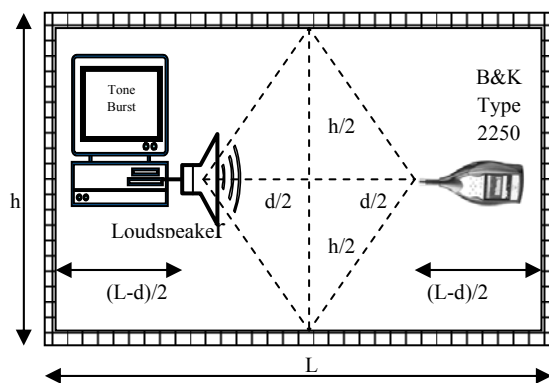
Fig. 3. The geometry environment
