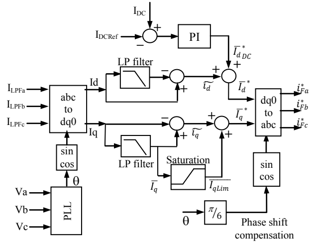
Fig. 7. Control Block
