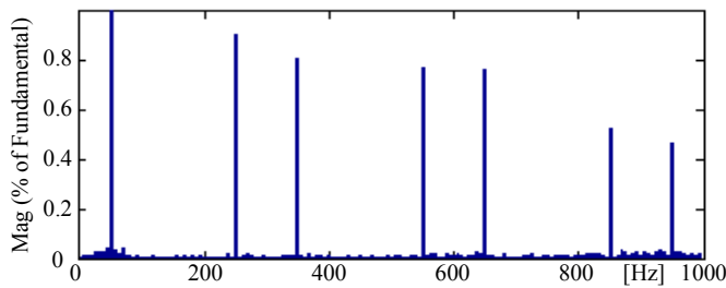
Fig. 11. System current spectra (Ia) with compensation. Fundamental 1422 A - THD= 1.83%.
