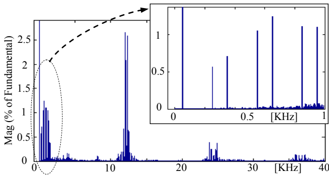
Fig. 10. System voltage spectra (Va) with compensation (and detail) Fundamental 10.78 kV - THD=3.10%.
