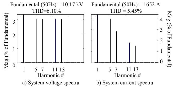
Fig. 2. System voltage and current spectra without compensation
